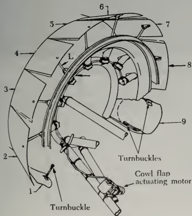
FIGURE 6-46. Cowl flap installation.
